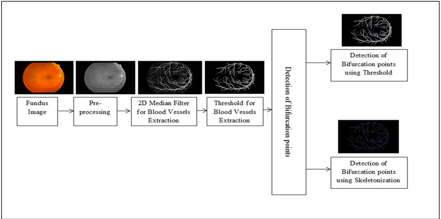
Figure 1: Flow chart for proposed algorithm of Extraction of the Retinal Blood Vessels and Detection of the Bifurcation Points
