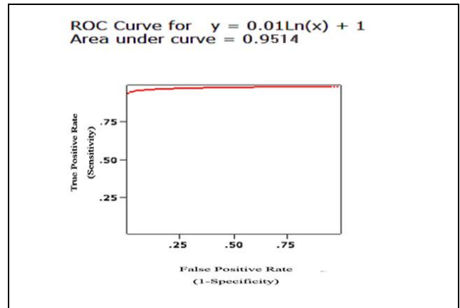
Figure 9: Receiver Operating Characteristics Curve for blood vessel extraction and detecting bifurcation points of vessels on online available Database diaretdb0
